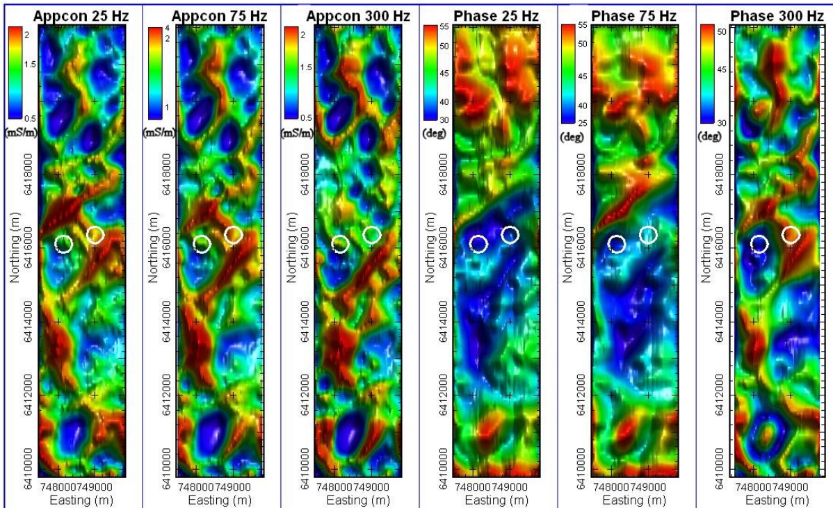
Figure 10: Apparent conductivities (left panels) and phases (right panels) derived jointly from ZTEM T xz and T zy responses 25-300 Hz. The location of the known conductors is indicated by white circles.
